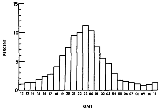
FIG. 4. Hourly percentage of tornado reports January 1968 through 15 June 1974. Graph indicates all tornadoes beginning during indicated hour (GMT).
