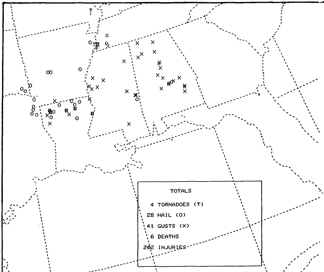
FIG. 3. As in Fig. 2, except from 1200 UTC 14 December 1987 to 1200 UTC 15 December 1987.
