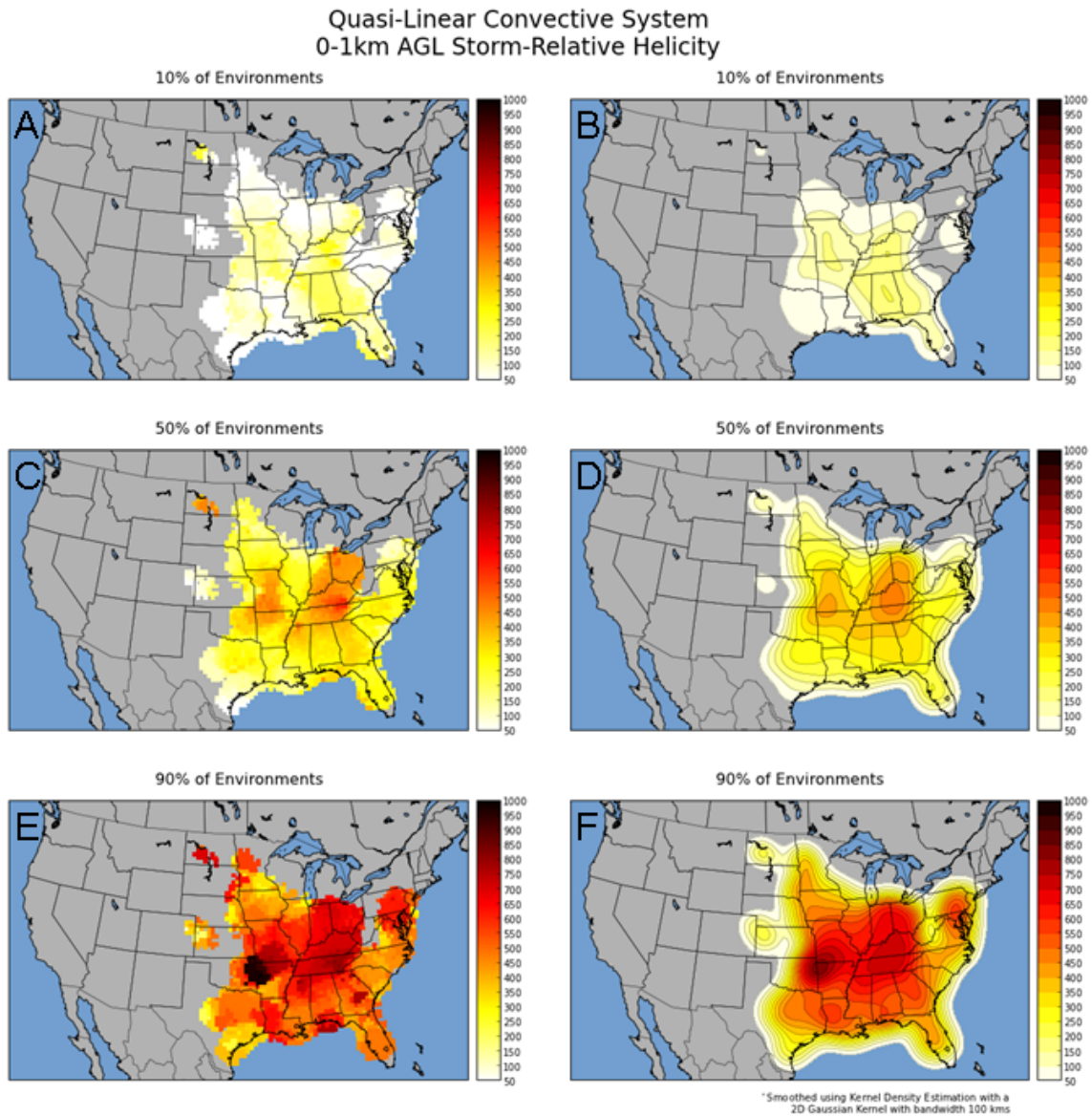
Figure 10. Same as Fig. 5, except for 0–1-km SRH ( m^2 s^{-2} ) associated with QLCS tornadoes.
