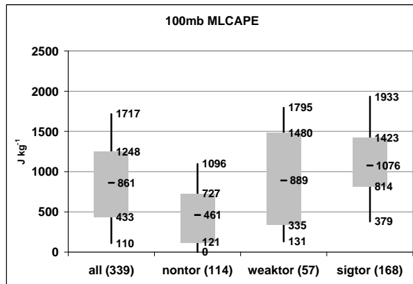
Fig. 18 Box and whiskers plot of MLCAPE ( \text{J kg}^{-1} ) for supercell grid hours for all supercells (339), non-tornadic supercells (nontor, 114), weakly tornadic supercells (weaktor, 57) and significantly tornadic supercells (sigtor, 168). The shaded box covers the 25 th -75 th percentiles, the whiskers extend to the 10 th and 90 th percentiles, and the median values are marked by the heavy horizontal line within each shaded box.
