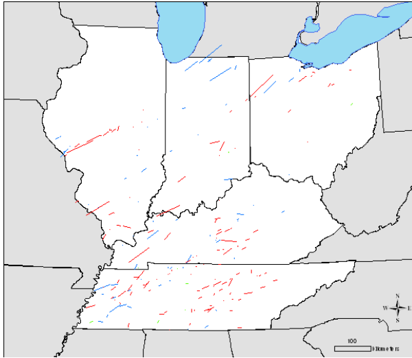
Fig. 12. Tornadoes by mode (supercell-red, QLCS-blue, other-green).
