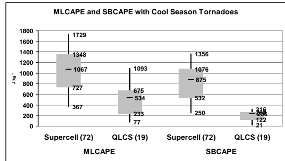
Fig. 15. Box and Whiskers plot of MLCAPE ( J kg^{-1} ) and SBCAPE ( J kg^{-1} ) for severe report grid hours for supercell tornado (72) and QLCS (19) tornado. The shaded box covers the 25 th -75 th percentiles, the whiskers extend to the 10 th and 90 th percentiles, and the median values are marked by the heavy horizontal line within each shaded box.
