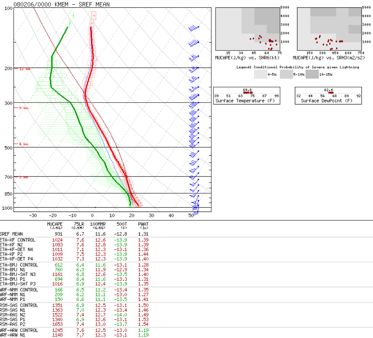
Figure 3. Composite diagram of mean SREF sounding and a table of thermodynamic statistics, 2-d graphs of each ensemble member (represented as a point) displayed over SPC climatological information, and 1-d graphs of each ensemble member (also represented as a point) of surface temperature and dewpoint.
