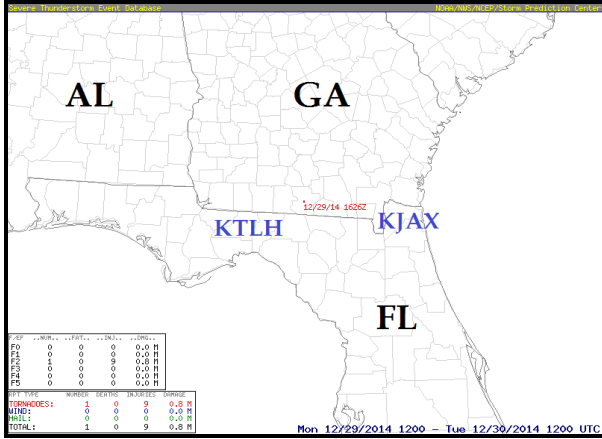
Figure 10. Valdosta, Georgia, EF2 tornado noted by red dot and related date/time. KTLH and KJAX denote the locations of the 1200 UTC observed soundings at Tallahassee and Jacksonville, Florida, respectively.
