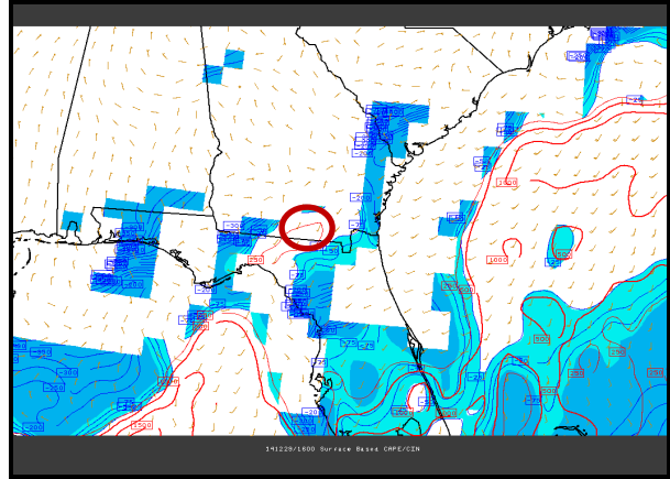
Figure 13. 1600 UTC 29 December 2014 SPC Mesoscale Analysis of surface-based CAPE/CIN.
