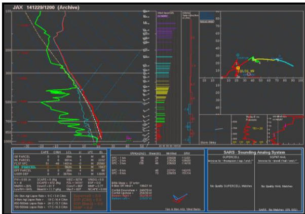
Figure 12. Observed sounding from Jacksonville, Florida (KJAX) on 12 UTC 29 December 2014.
