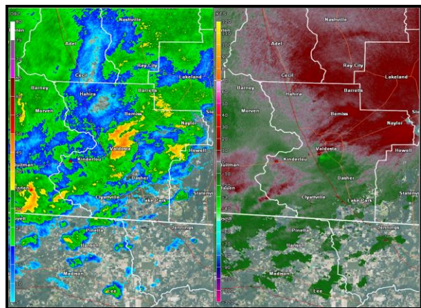
Figure 14. 1.4 degree reflectivity (left) and storm-relative velocity (right) WSR-88D radar imagery from Moody Air Force Base, Georgia, (KVAX) at 1621 UTC 29 December 2014.
