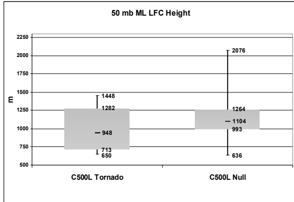
Fig. 9. Same as Fig. 2, except 50 mb ML LFC Height (m).
