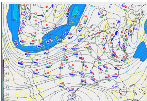
Fig. 1. 300 mb objective analysis for 0000 UTC 23 June 2003. Streamlines are in black. Blue shading denotes wind speeds of 75 knots or greater.
