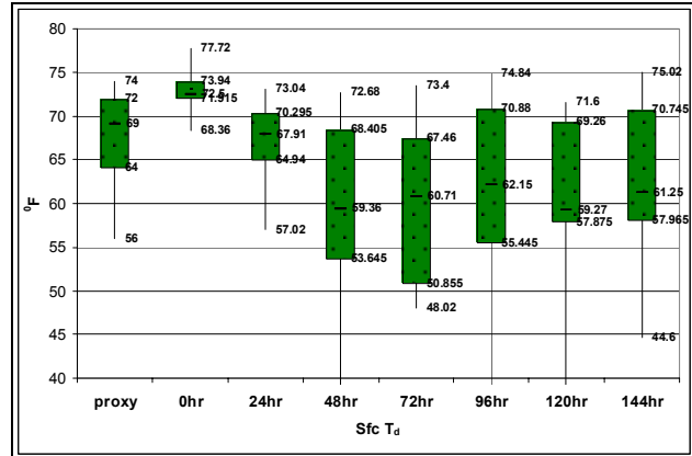
Fig 3. Same as Fig. 2a but for buoy 42019.
