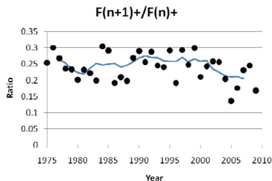
Figure 2: Average number of tornadoes of at least F(n+1) damage divided by at least F(n) damage, averaged over n=1 to 3, by year (black dots) for 1975-2009. Five-year running value shown by blue line.
