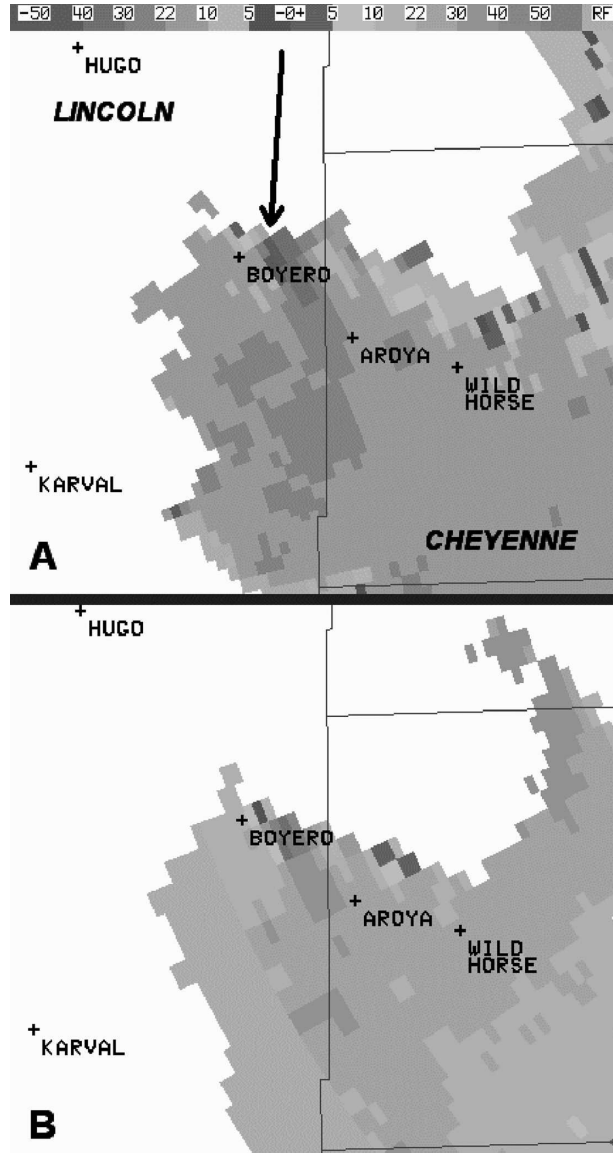
FIG. 5. The 0.5° elevation angle SRM displays at 0034 UTC 16 Jun 2002, from (a) PUX and (b) GLD. County names, arrow pointing toward mesoanticyclone center, and the velocity gray-scale each are provided in (a). Locality names appear on both images, which are scaled identically. PUX and GLD radars were located generally southwest of (a) and northeast of (b), respectively. Velocities are shown in kt (1 kt ≈ 0.5144 m s -1 ).
