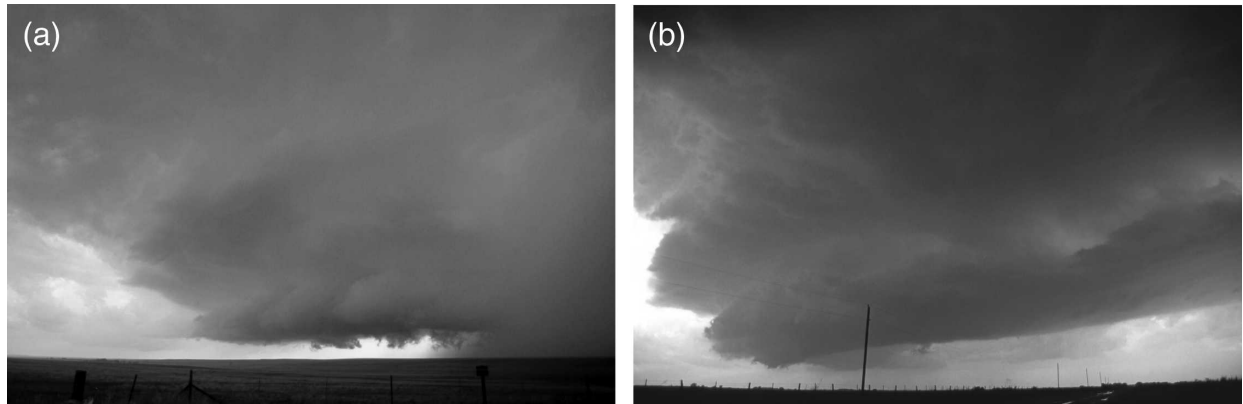
FIG. 9. Visual storm structure comparison using monochrome photographs of (a) the nontornadic, anticyclonic Aroya supercell from 15 Jun 2002, mirrored as if to look toward the southwest, and (b) the incipiently tornadic, cyclonic Dover supercell of 4 Oct 1998, with actual view to the southwest.
