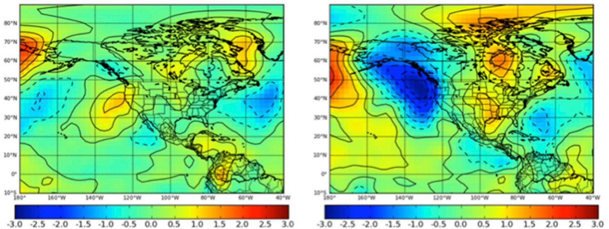
FIG. 6. Monthly anomalies of 850-hPa V -component wind ( m s^{-1} ) during January (left) El Niño and (right) La Niña conditions.
