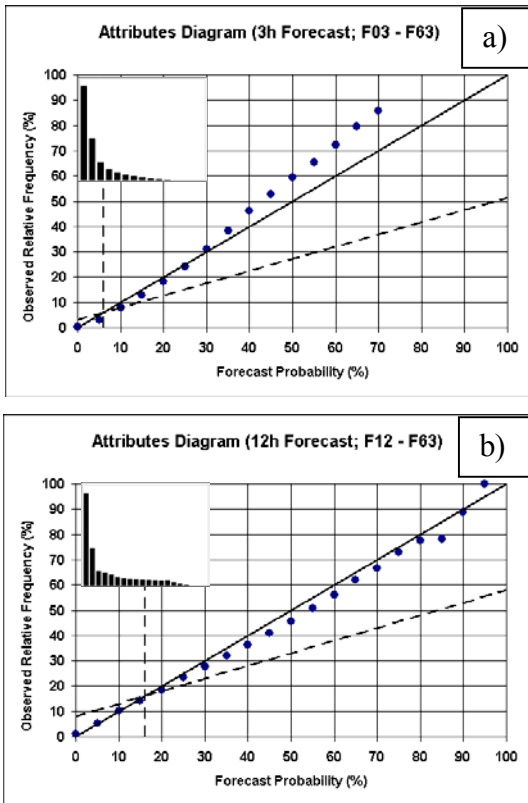
Fig. 3. Attributes diagrams for the calibrated probability of a thunderstorm over the United States at (a) 3h intervals and (b) 12h intervals. Verification period is 15 April 2005 through 15 October 2005. Inset represents the relative frequency of each forecast interval.
