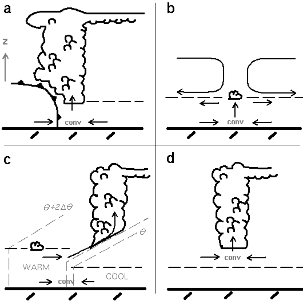
Fig. 2 Schematic of subcloud horizontal mass convergence (conv) as it relates to cumulus convection (represented by cloud outline). Arrows represent streamlines. Thick dashed line indicates top of PBL. (a) Surface horizontal mass convergence maximum is associated with a deep tropospheric circulation and deep moist convection. (b) Surface horizontal mass convergence maximum is associated with shallow cumulus development owing to midlevel subsidence and/or a capping inversion. (c) Surface horizontal mass convergence maximum is
